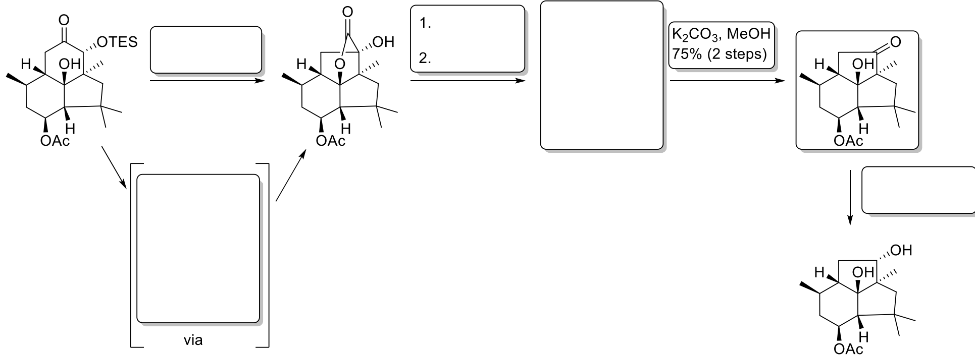
4β-Acetoxyprobotryane-9β,15α-diol
